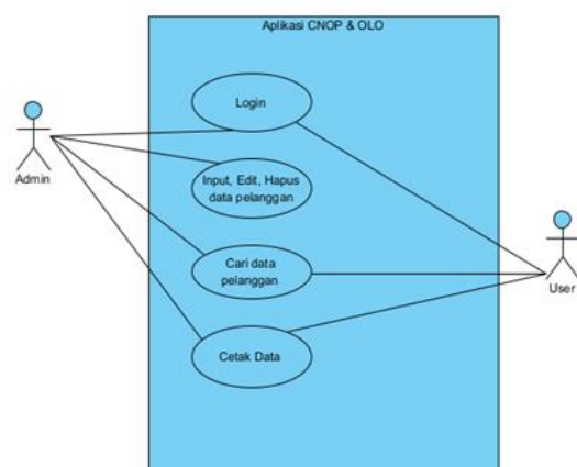
Gambar 1 Usecase Diagram
